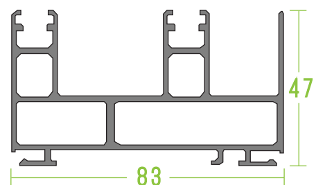
SLIDING TRACK DIMENSIONS AS 39 NI TROPTEC - DOUBLE TRACK
