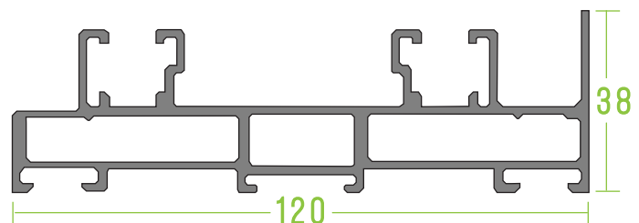
SLIDING TRACK DIMENSIONS ASS 50 NI - DOUBLE TRACK
